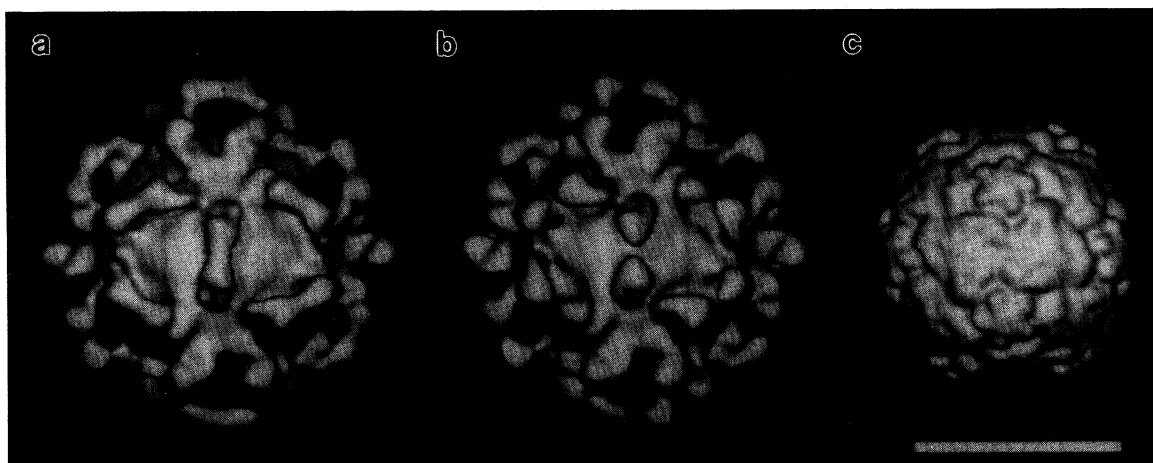
FIG. 2. Three-dimensional reconstructions of the IgG-virus complex ( a ) and of the Fab-virus complex ( b ) and a surface representation of the atomic map of HRV14 ( c ) truncated to 20-Å resolution. The surface representations in a and b were calculated at equivalent contour levels. (Bar = 250 Å.)
